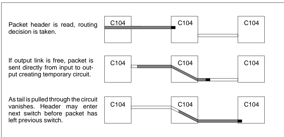
Figure 3.3 Wormhole routing
