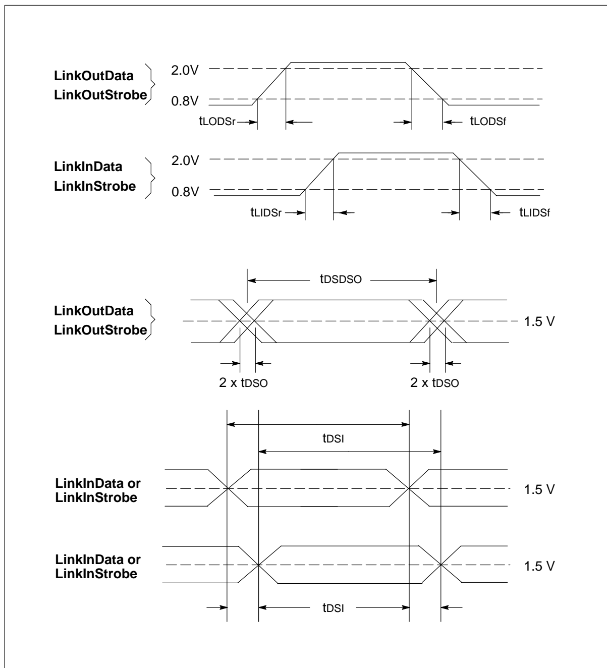
Figure 11.2 DS-Link timing
