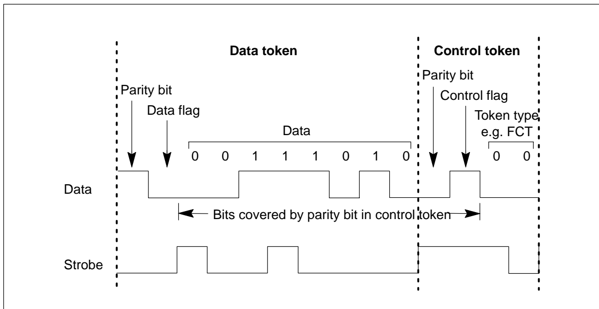
Figure 6.1 Link data and strobe formats
