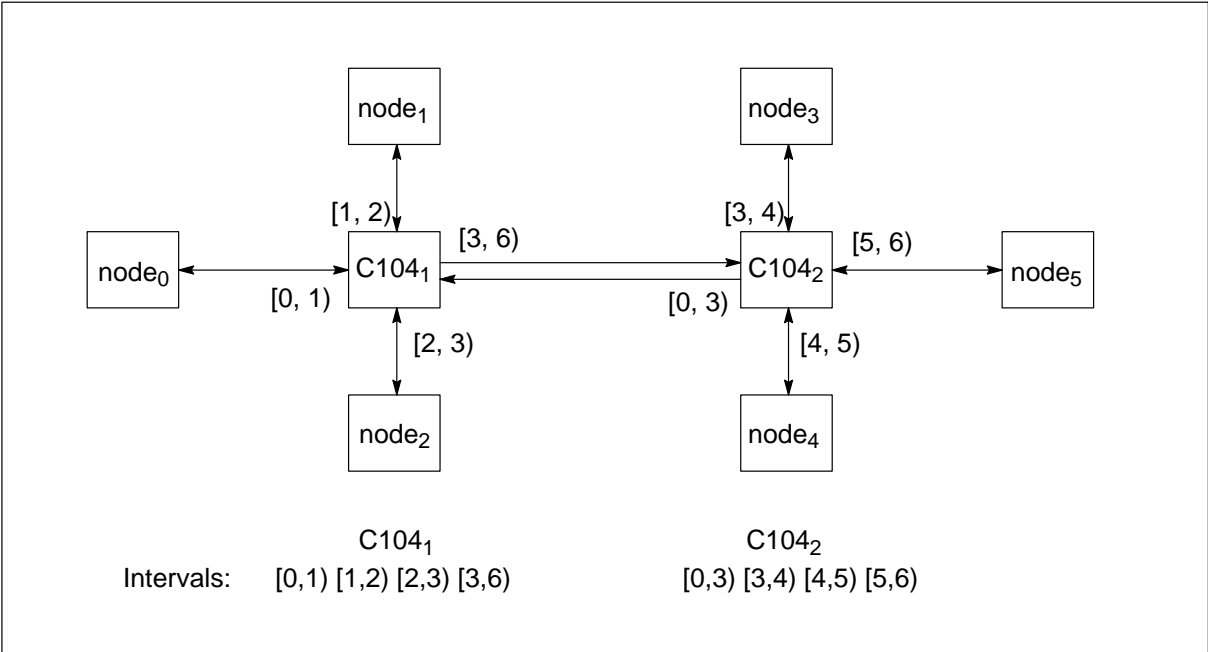
Figure 3.5 Interval routing
