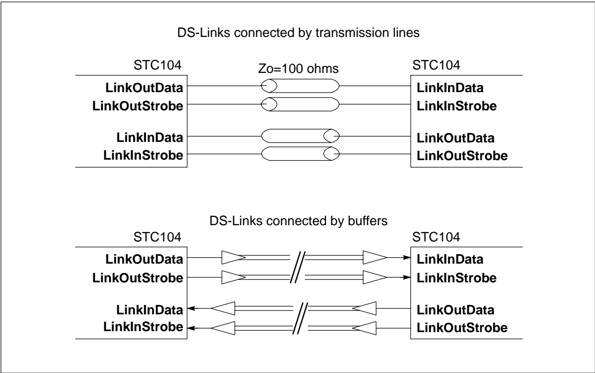
Figure 6.2 DS-Link connections
