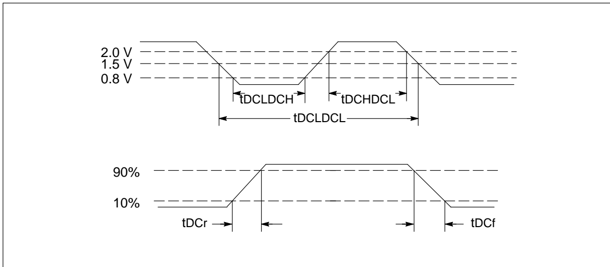
Figure 11.1 ClockIn timing
