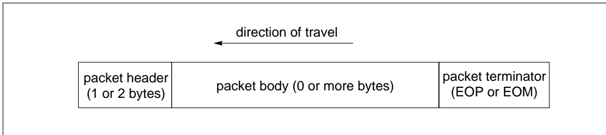
Figure 3.2 Packet structure
